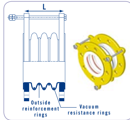
BELLOWS RANGE VACUUM V207 Available only with 3 convolutions
