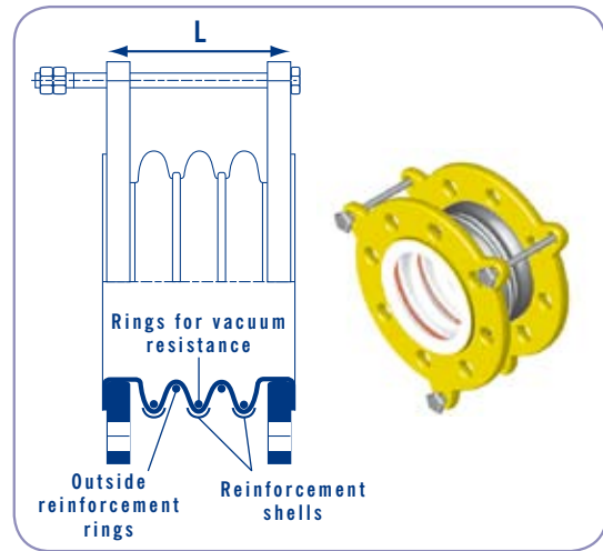
BELLOW RANGE VACUUM V227 3 convolutions only
