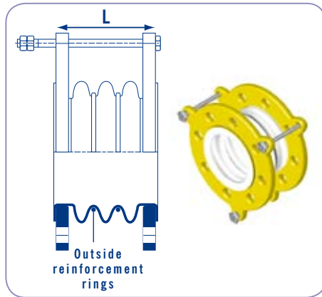
BELLOWS STANDARD RANGE G207 3 and 5 convolutions
