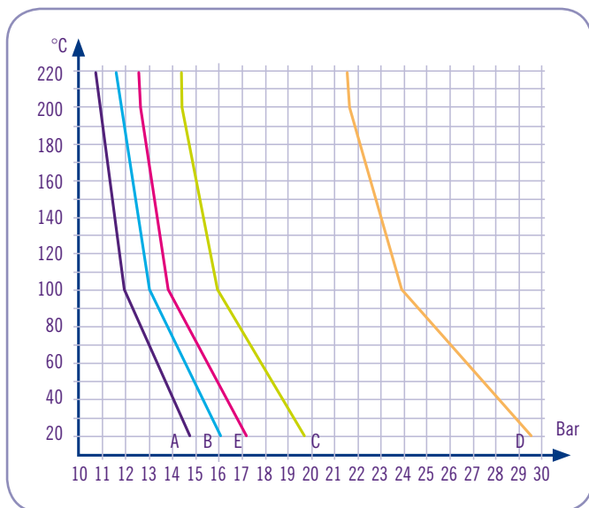
PRESSURE RESISTANCE
