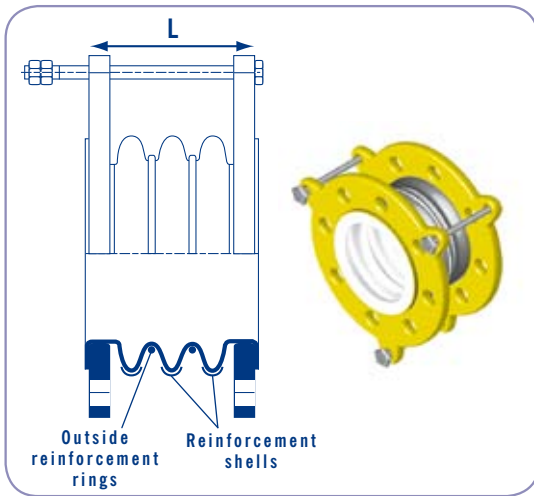
BELLOW STANDARD RANGE G227 3 convolutions only
