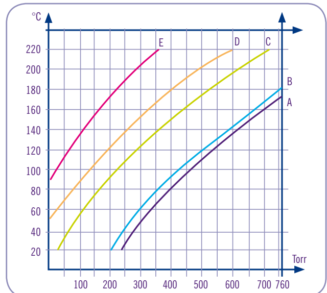
VACUUM RESISTANCE
