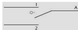
3 position change-over disconnectors (1-0-2)
