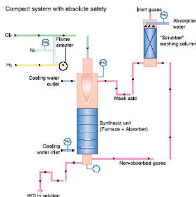
HCl synthesis unit
